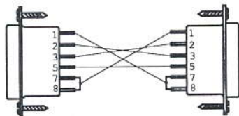
9-pin to 9-pin
