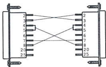
25-pin to 25-pin
