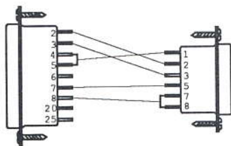
25-pin to 9-pin
