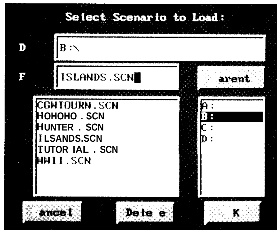
Figure 4: File Requester
