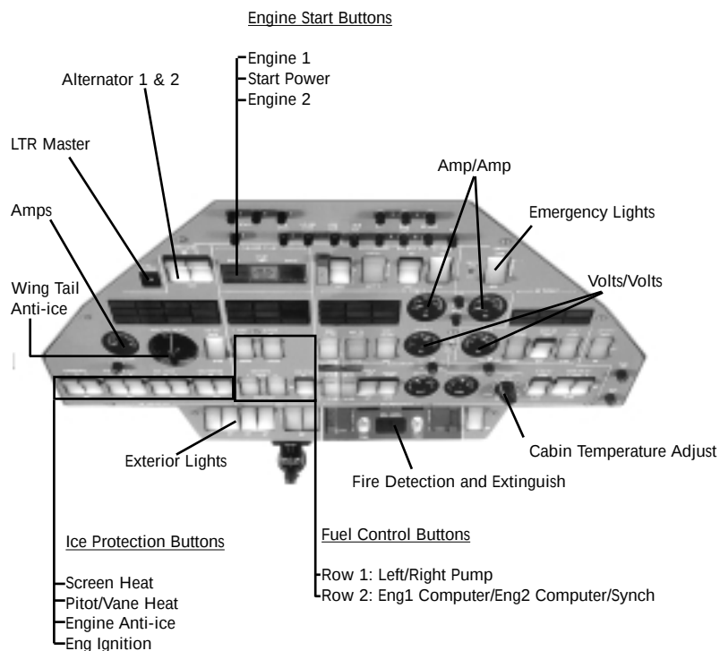
Hawker 800XP Ceiling Instrument Panel
