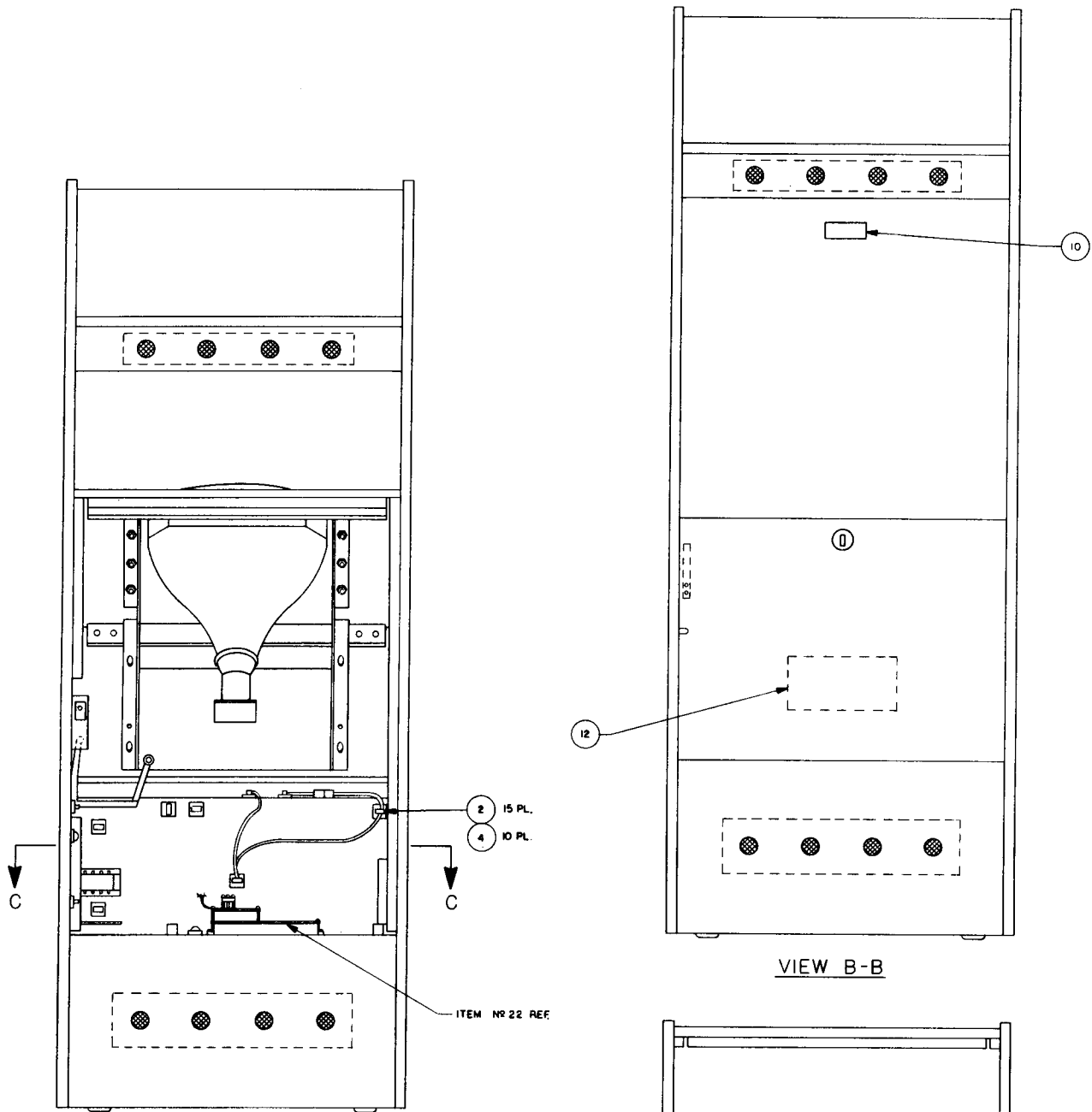
VIEW B-B (W/ REAR PANEL AND DOOR REMOVED)
