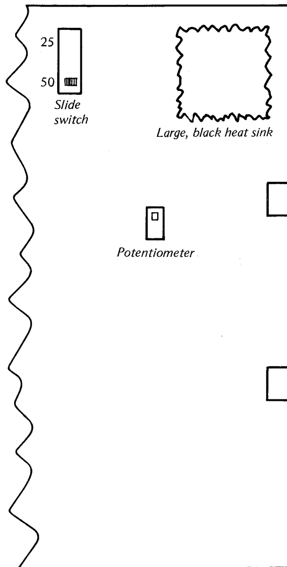
Figure 4-1 Location of Players-per-Coin Switch and Game Time Potentiometer
