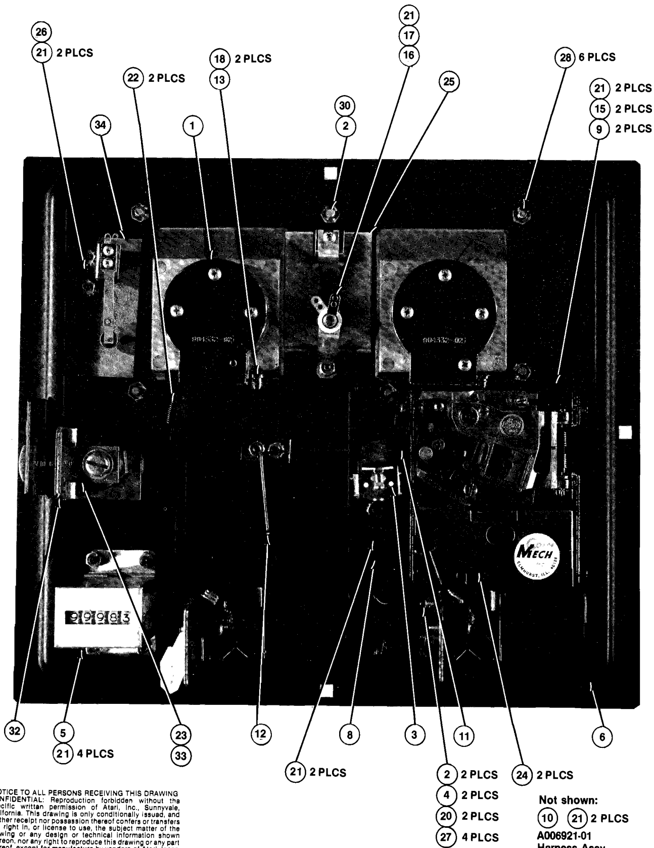
Figure 18 Coin Door Assembly A006794-16 thru -27 J
