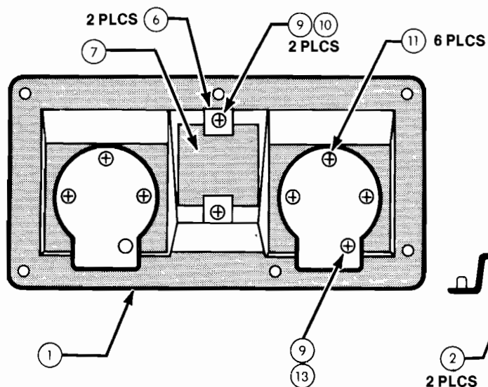
Figure 19 Front Bezel Assembly A007637-16 thru -27 G
