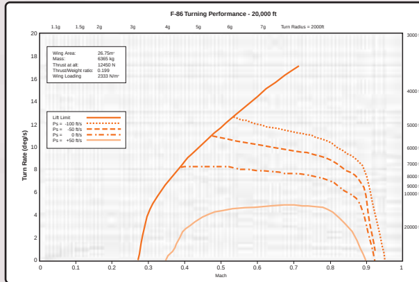
Fig 1: F86E, 20,000ft
