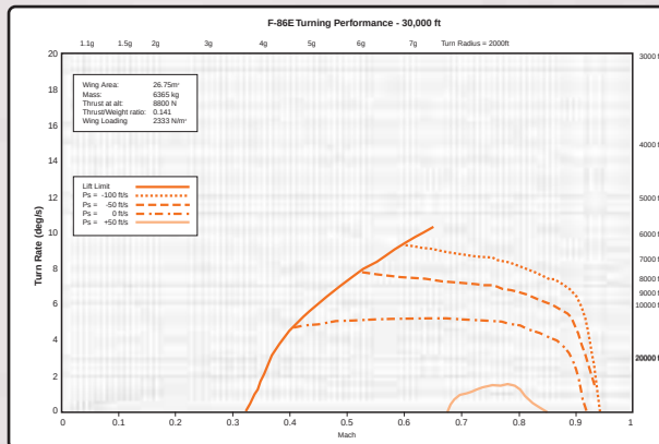
Fig 2: F86E, 30,000ft
