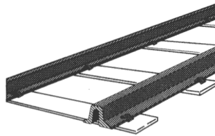
U-Profil, 1844
