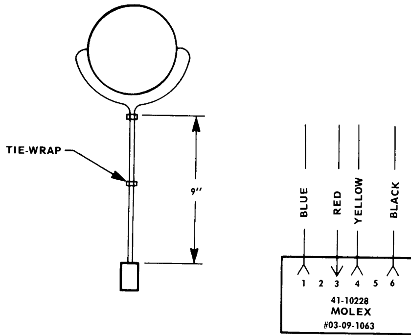
40-10268 YOKE, BROY #746
