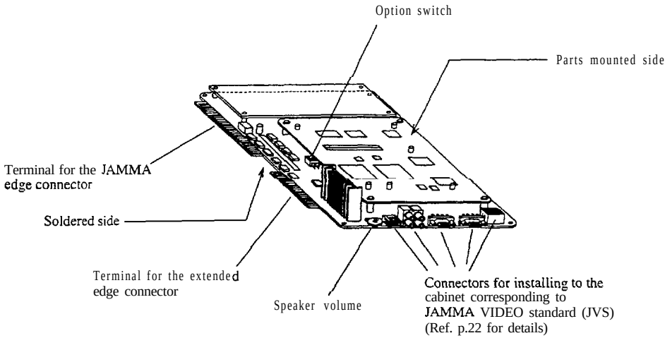
PC Board
