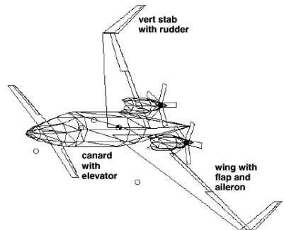
The Beech Starship has a vertical stabilizer at each wingtip and a canard as it's horizontal stabilizer
